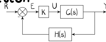
Figure def.1: a block diagram for a proportional controller K .
