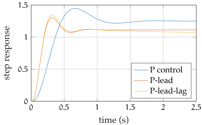
Figure multd.3: step responses for proportional, proportional-lead, and proportional-lead-lag controllers.
