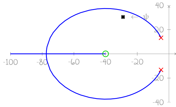
Figure PID.1: root locus without compensation.
