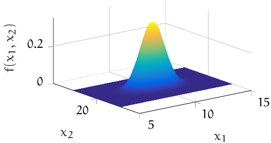
Figure multivar.1: two-variable gaussian PDF.
